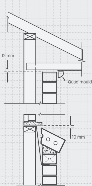
FIGURE 4.20 SHRINKAGE ALLOWANCE FOR TIMBER FRAMING
